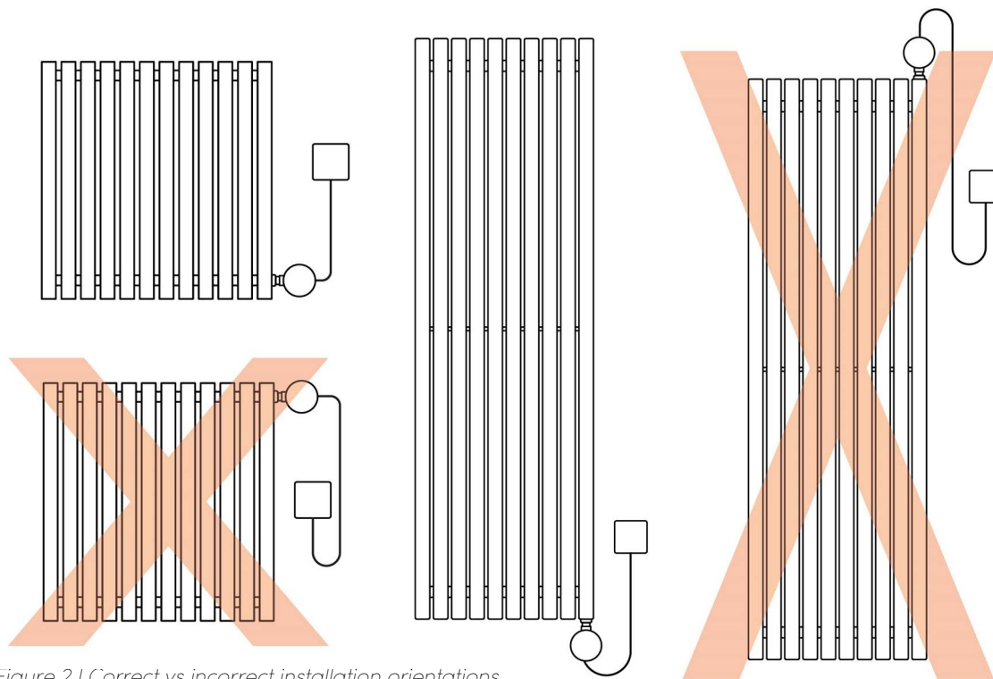
Figure 2 | Correct vs incorrect installation orientations
