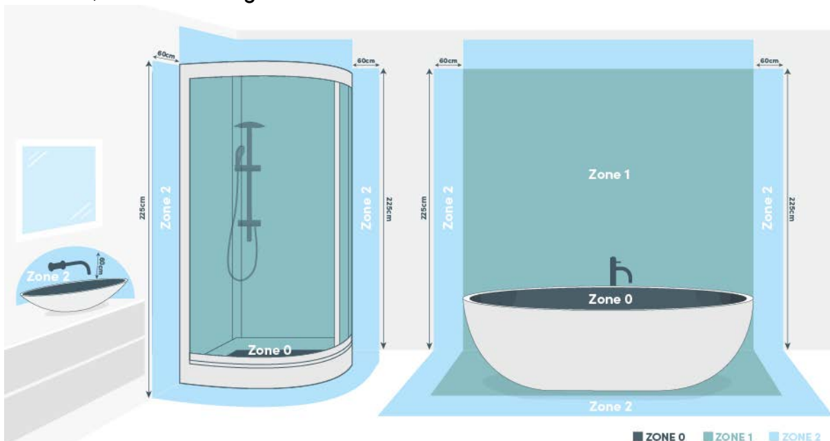
Figure 1 | Bathroom installation zones
